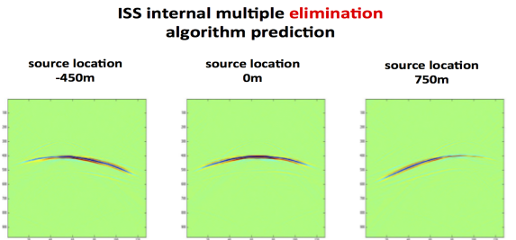
Figure 4: ISS internal multiple elimination algorithm prediction
