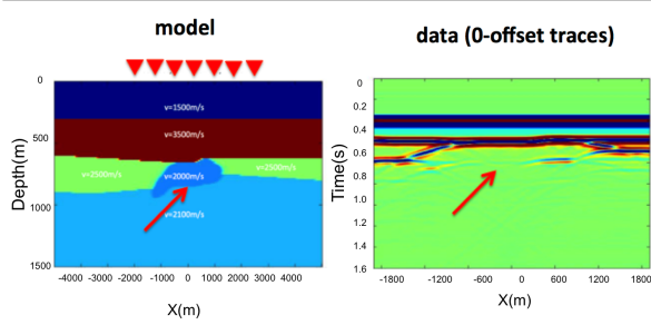
Figure 5: Zero offset traces of data. Note the interfering internal multiple and base salt primary.
