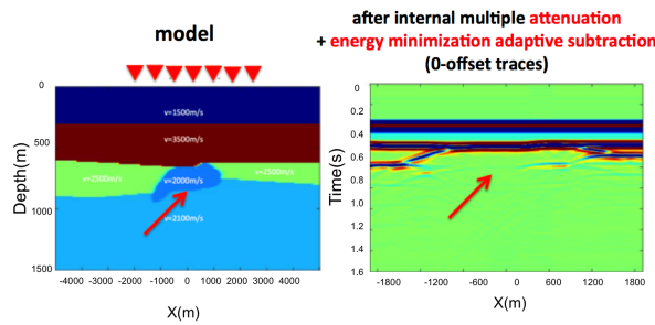
Figure 6: Zero offset traces after ISS internal-multiple attenuation and energy minimization adaptive subtraction. Note the damaged base salt primary.
