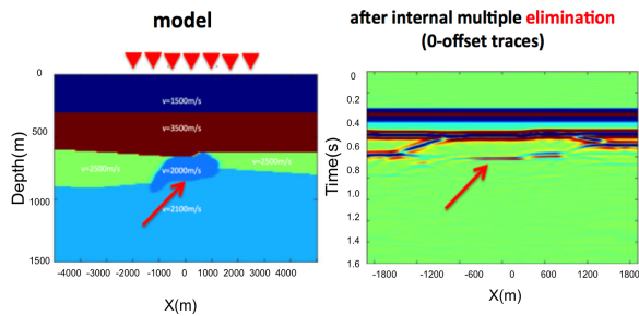
Figure 7: Zero offset traces after ISS internal-multiple elimination. Note the preserved base salt primary.
